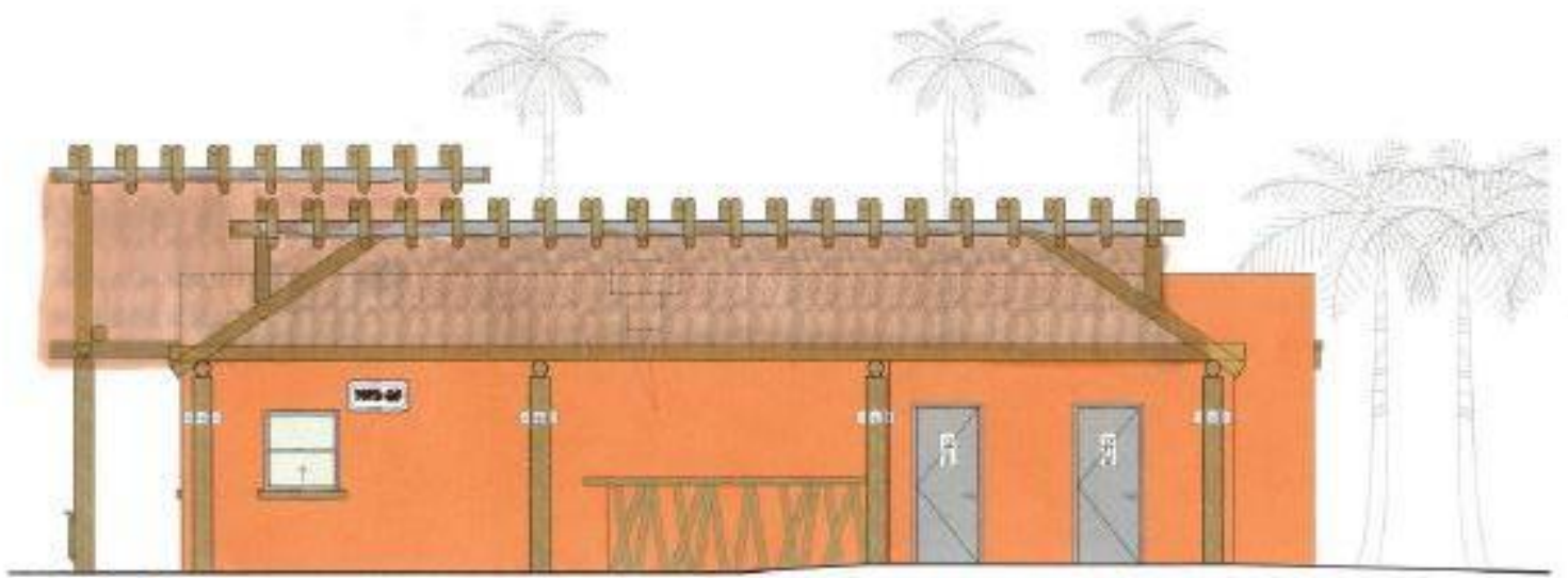
WEST ELEVATION
